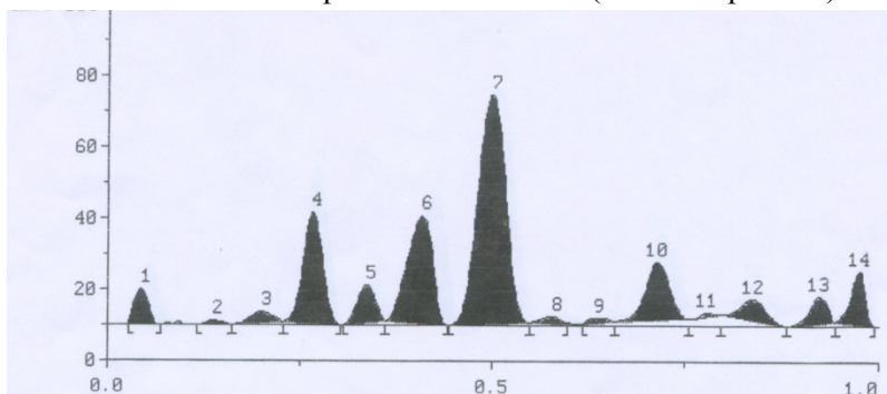
Fig.1: Typical HPTLC Chromatogram for Root Bark powder of A. mexicana .
